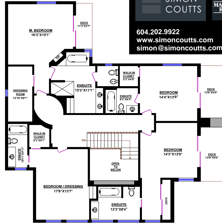
UPPER LEVEL
